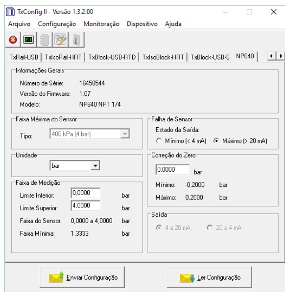
Figura 4 – Tela principal do software TxConfig-II
